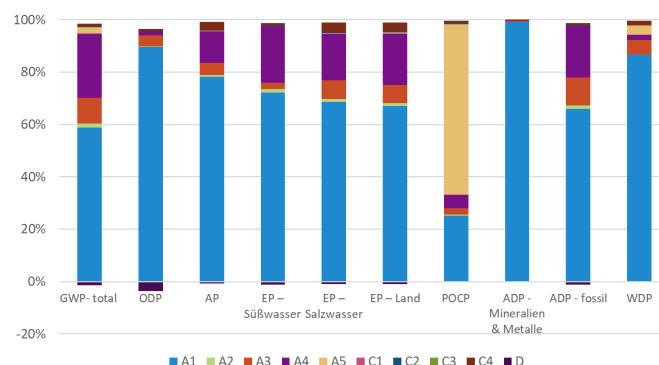
Figure: Influence of life cycle phases on the environmental impact of silicone resin plasters
